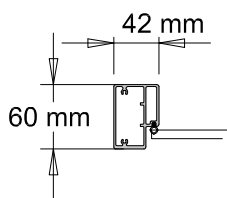
Aluminium frame
