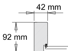
Aluminium frame
